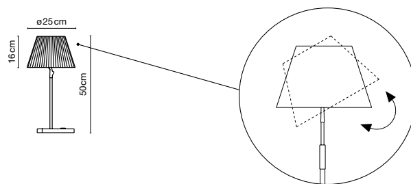
Balancing lampshade
