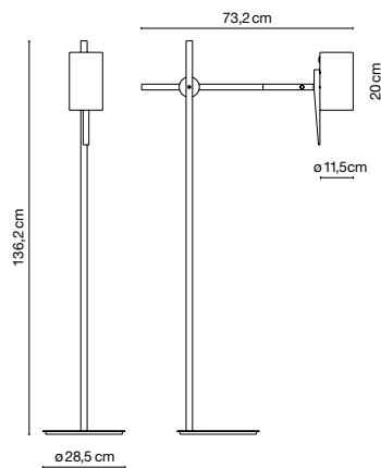
Scantling P73
