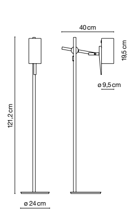
Scantling P40
